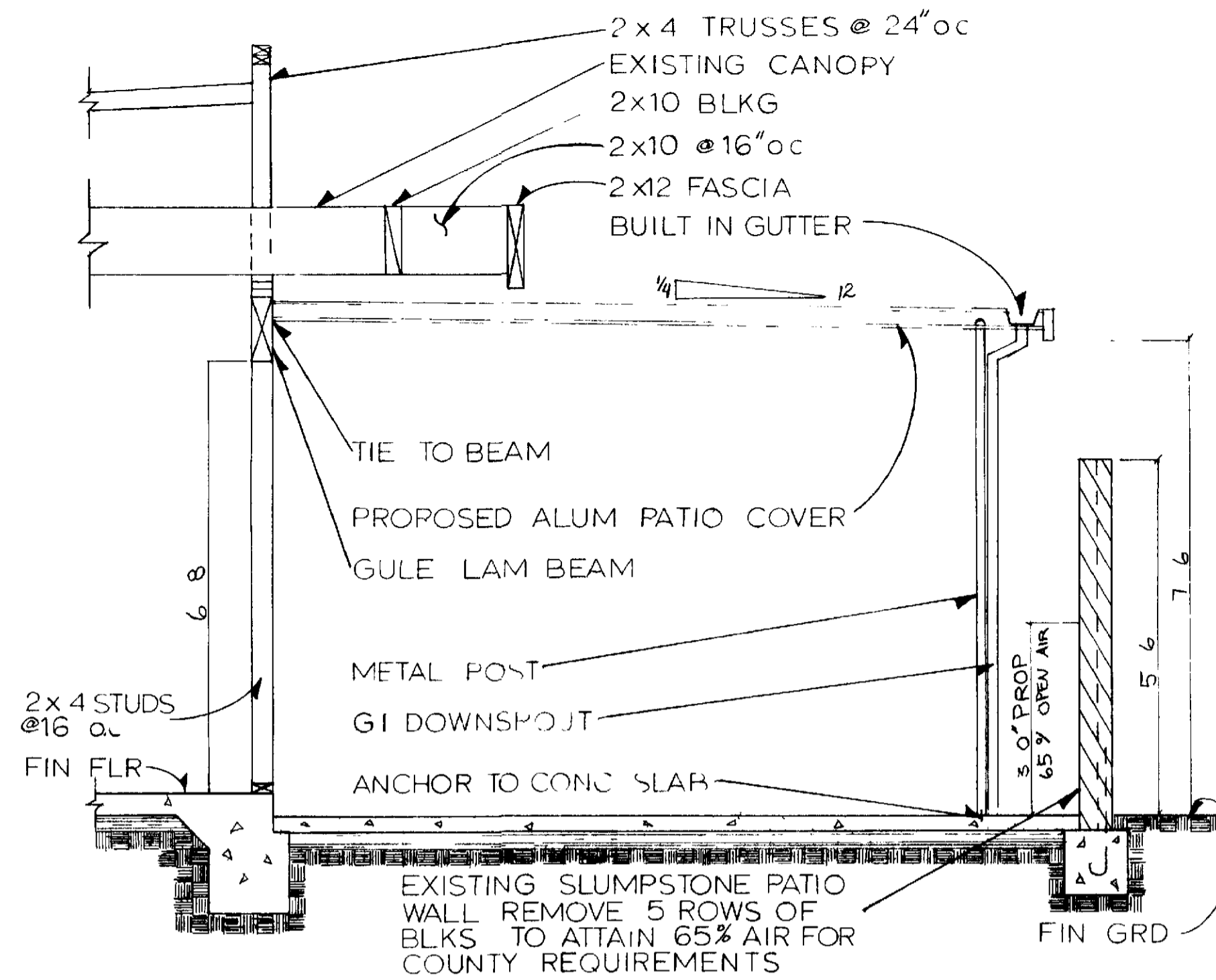
SECTION A-1 SCALE 1/2"=1'-0"
