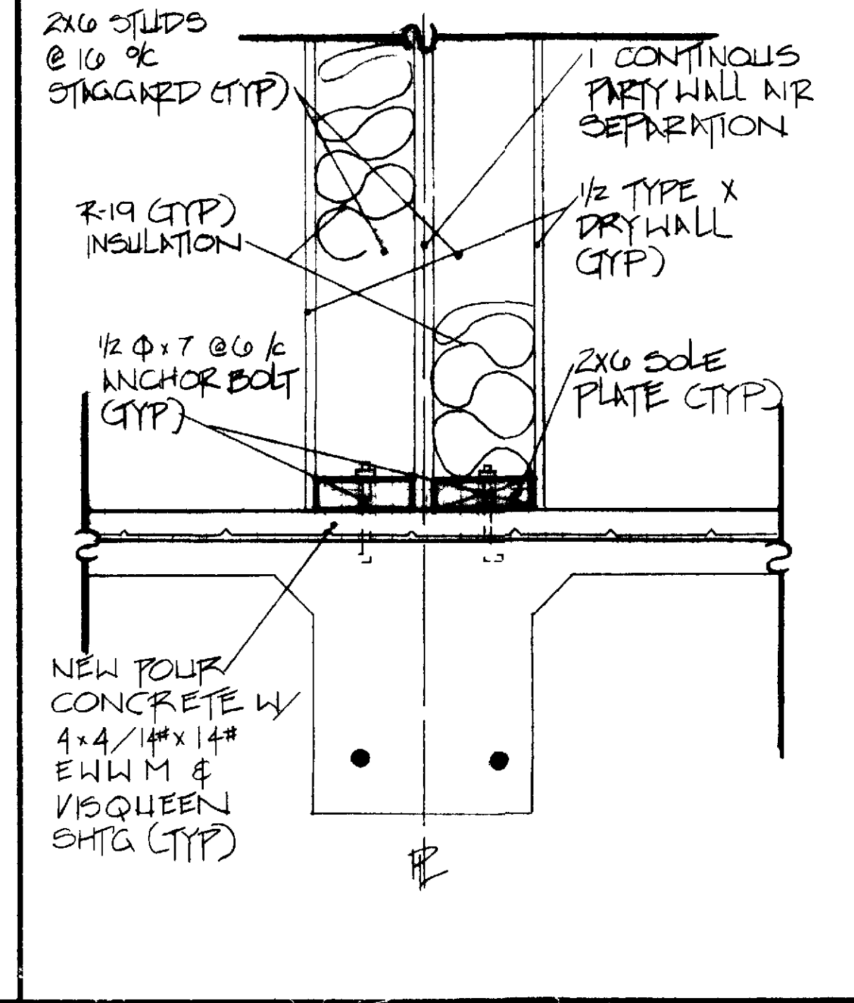
DETAIL SCALE 1/2" = 1'-0"
