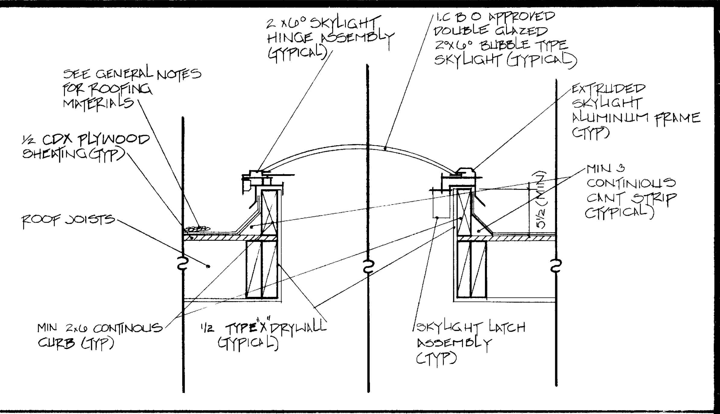
DETAIL SCALE 1-1/2" = 1'-0"
