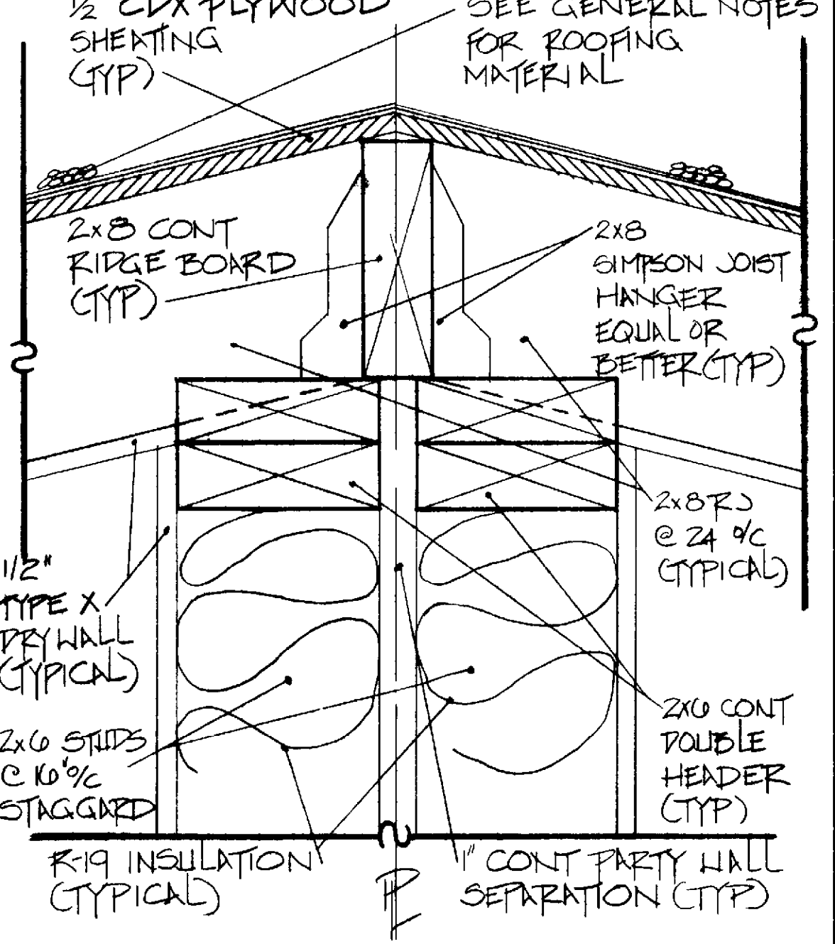
DETAIL SCALE 3/8" = 1'-0"
