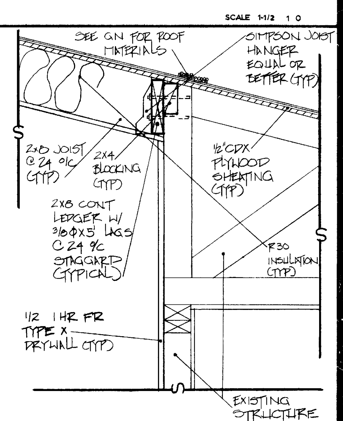
DETAIL SCALE 1/2" = 1'-0"
