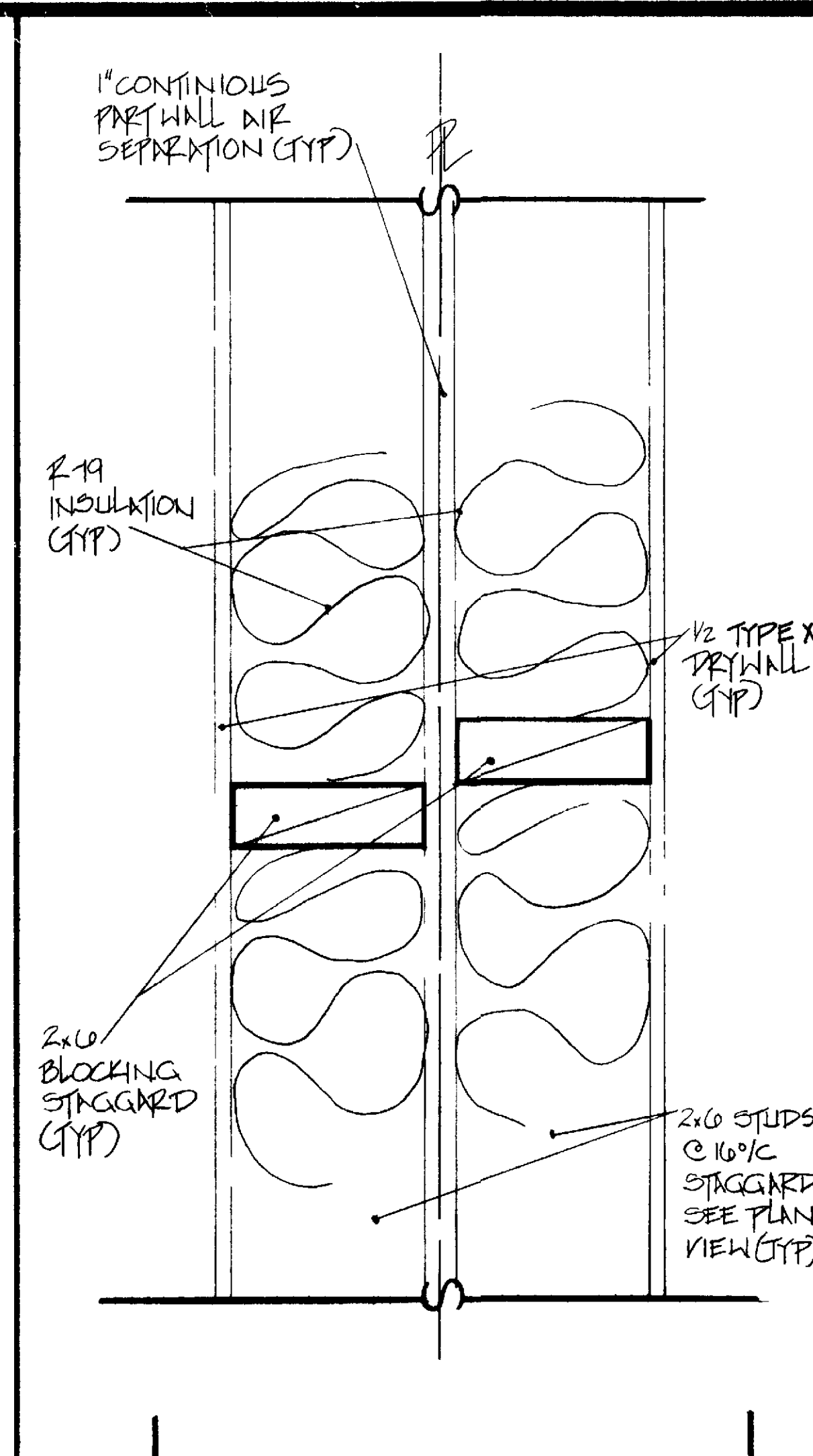
DETAIL SCALE 1-1/2" = 1'-0"
