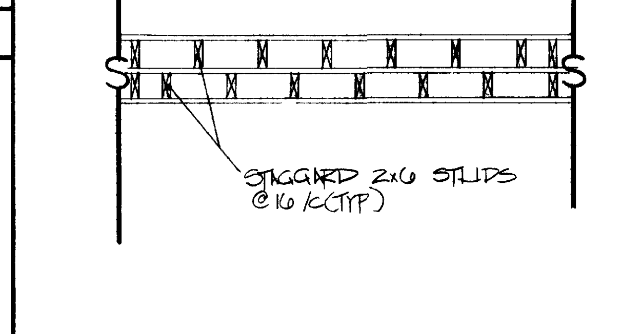
DETAIL SCALE 3/8" = 1'-0"
