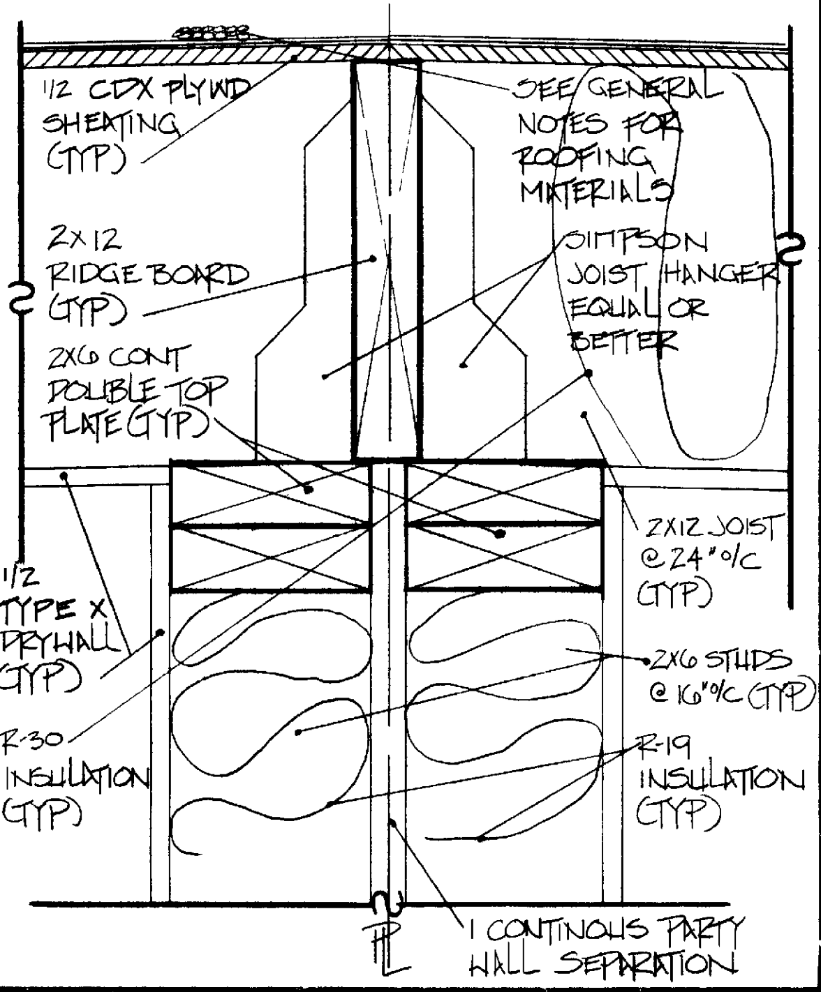
DETAIL SCALE 1-1/2" = 1'-0"
