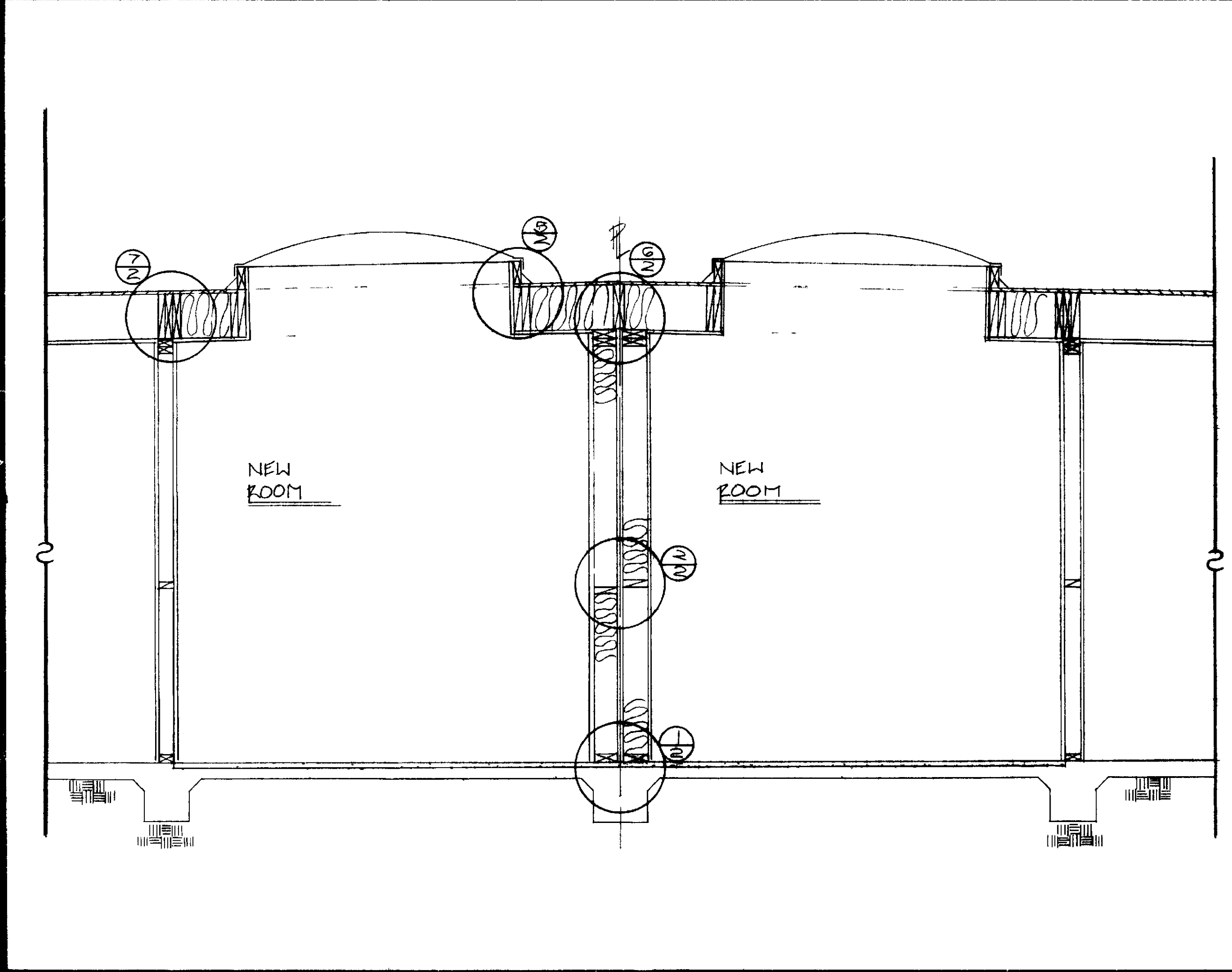
BUILDING SECTION 10B SCALE 1/2" = 1'-0"
