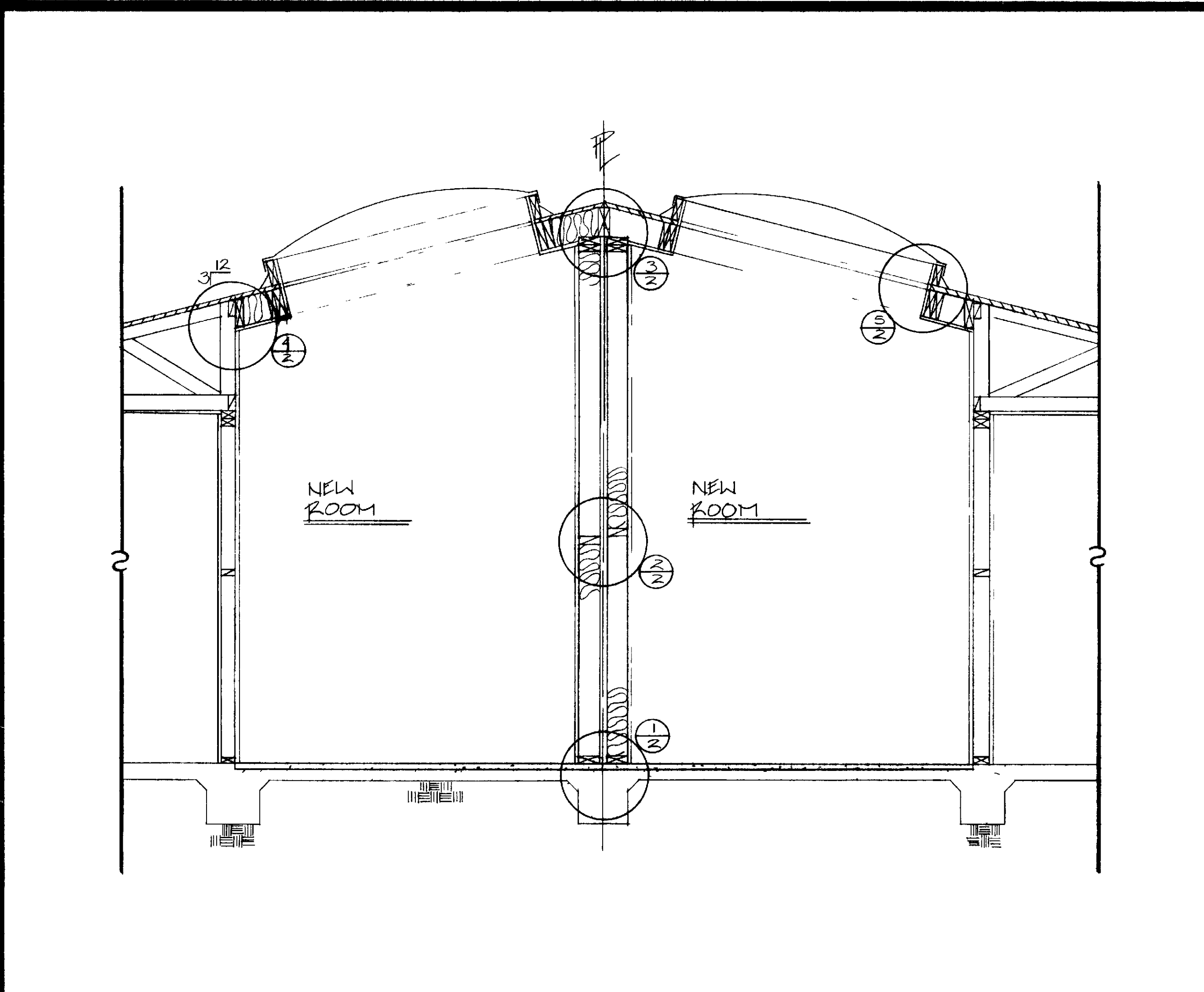
BUILDING SECTION 10A SCALE 1/2" = 1'-0"
